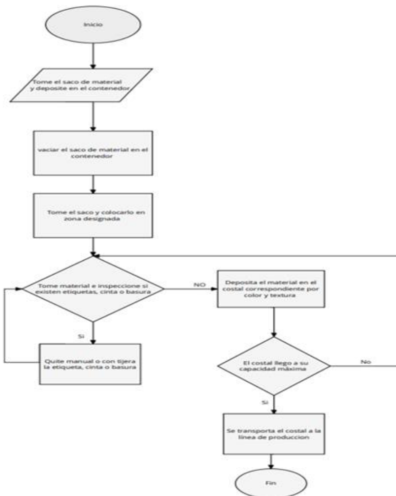
Figure 3. Flowchart
